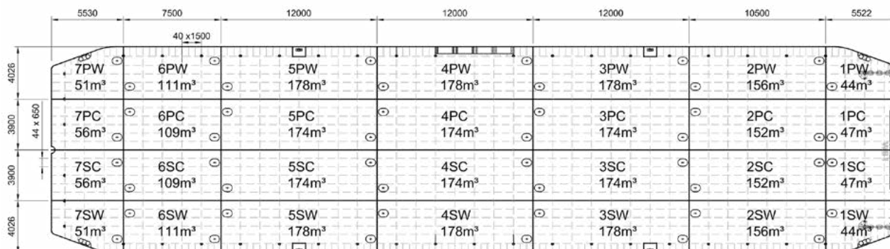
DECK AND STRUCTURAL LAYOUT
